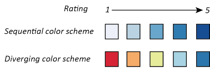
Figure 3: Color scheme for the rating. The diverging color scheme is finally chosen to emphasize both the higher and lower ratings.
